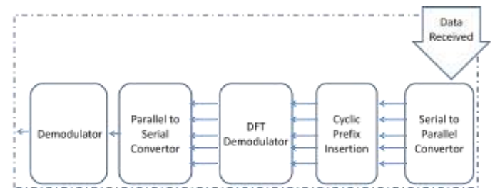
Figure 2 Receiver of OFDM
